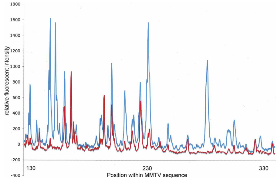
Figure 5. Example of an aligned primer extension capillary electrophoresis fluorogram trace. Raw fluorescence data from an ABI3730xl sequencer were aligned to ABI GeneScan500 molecular weight markers. Bare genomic DNA is in red, and internucleosomally cleaved DNA is in blue.
